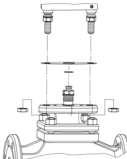
Fig. 9: Form C: mounting on rods
