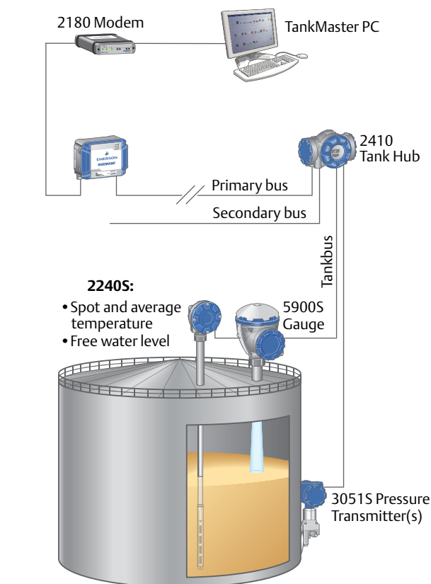
Rosemount 2240S Multi-input Temperature Transmitter installed together with a sensor
