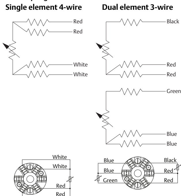
Figure 2. Sensor Lead Wire Termination - Pipe Clamp RTD Spring Loaded
