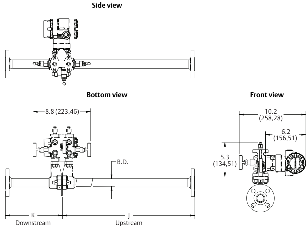
Figure 20. Rosemount 2051CFP Integral Orifice Flowmeter
