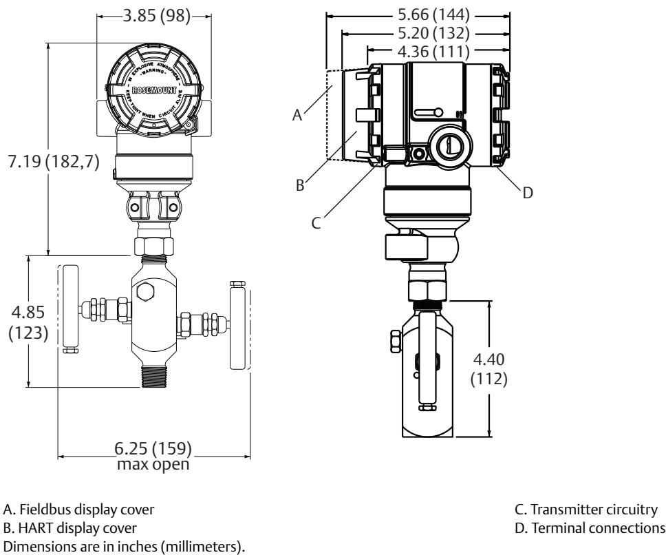
Figure 16. Rosemount 2051T with Rosemount 306 Two-Valve Integral Manifold
