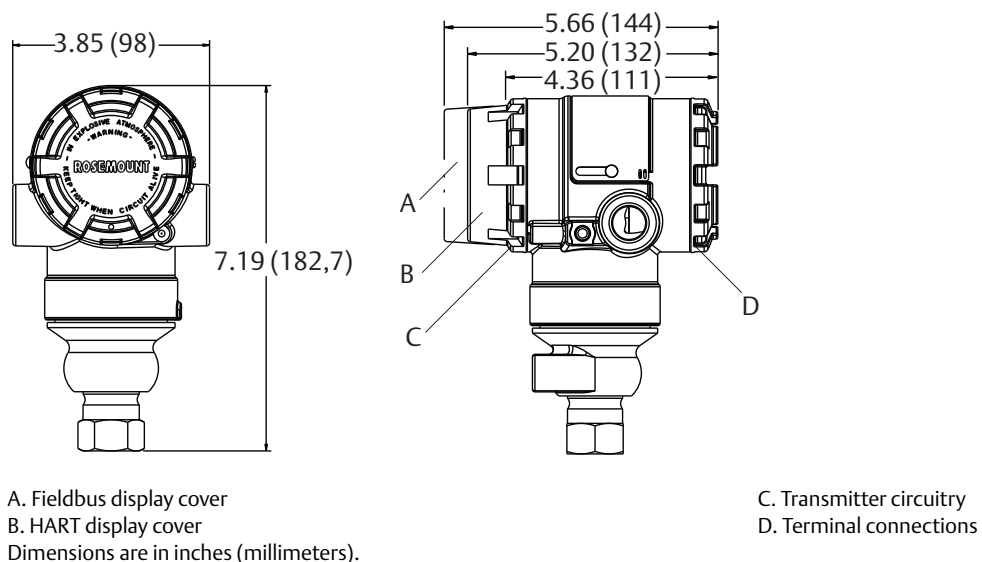
Figure 9. Rosemount 2051T
