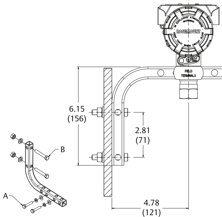
Figure 14. Rosemount 2051G with Optional Mounting Bracket
