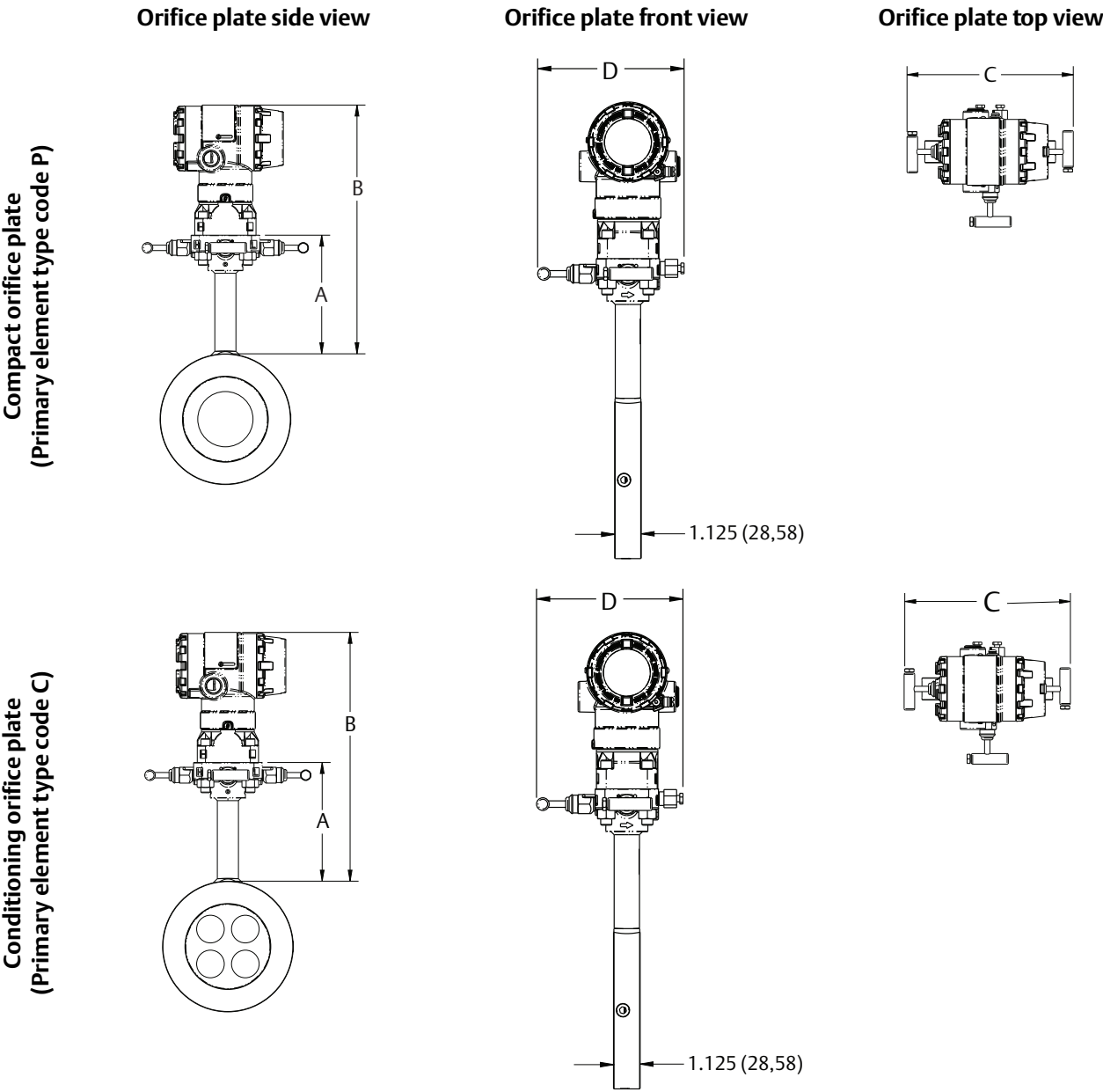
Figure 19. Rosemount 2051CFC Compact Orifice Flowmeter
