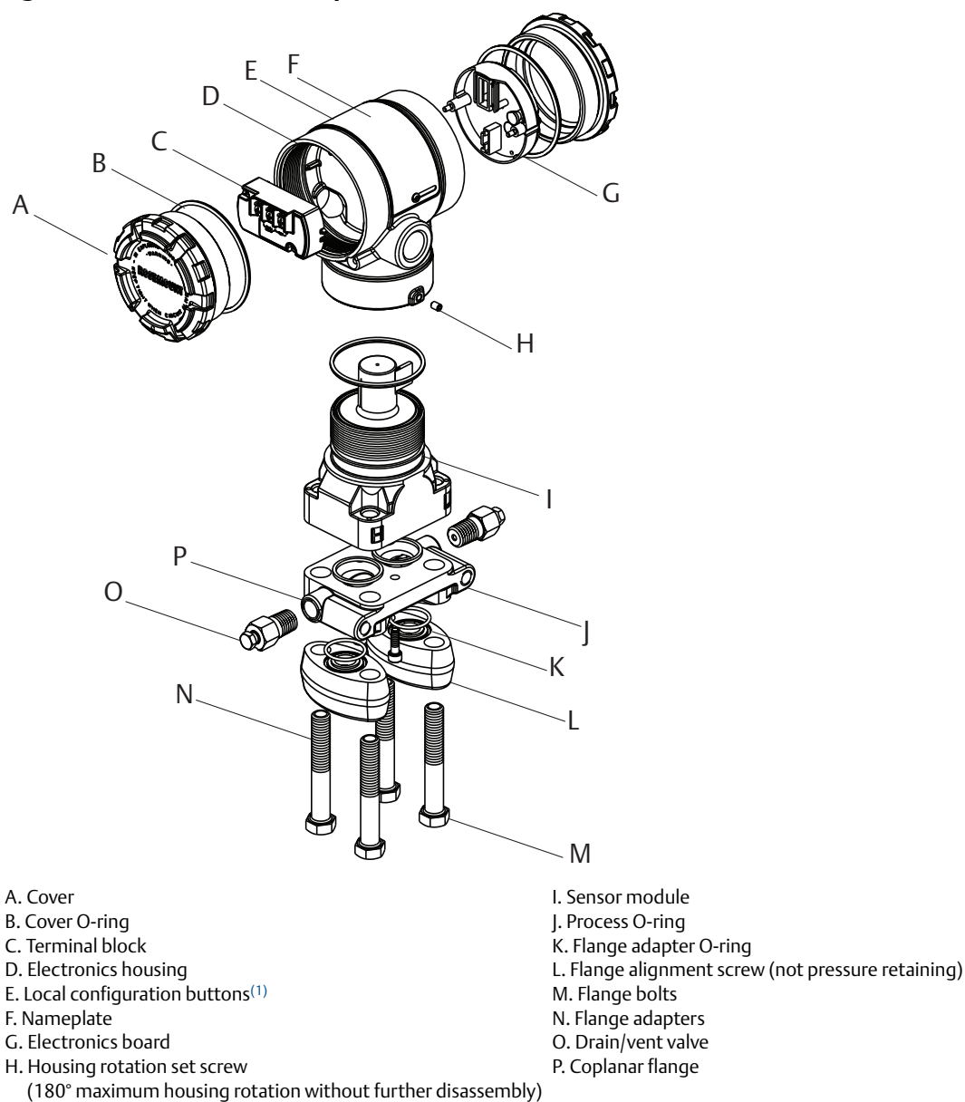
Figure 1. Rosemount 2051C Exploded View
