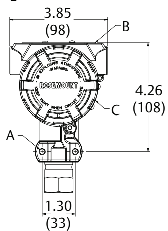
Figure 12. Rosemount 2051G Nameplate and Labels
