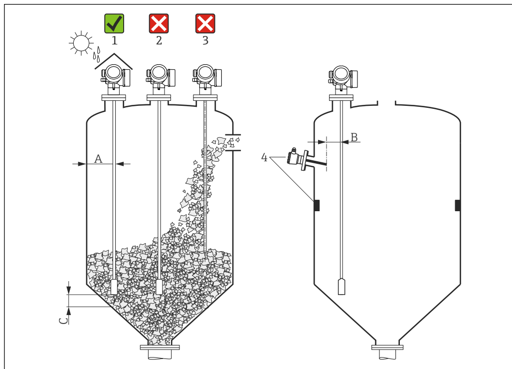
20 Mounting requirements for Levelflex
