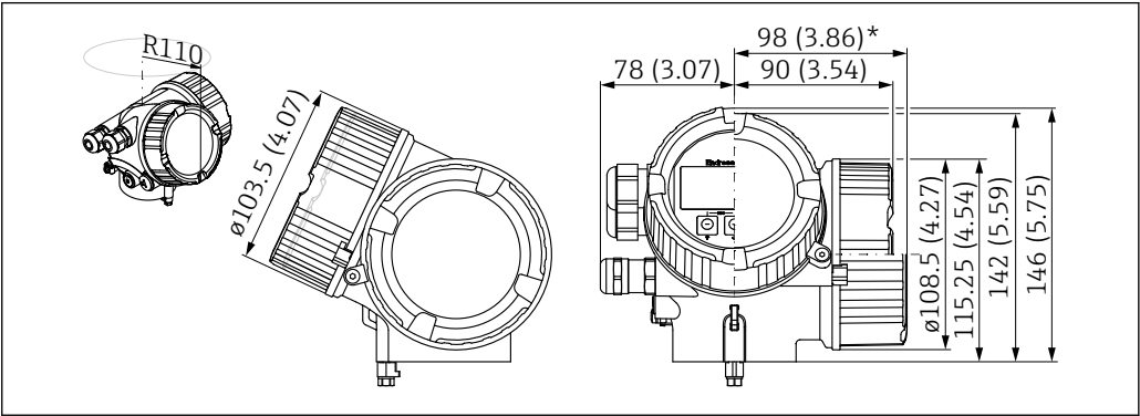
28 Housing GT18 (316L); Dimensions in mm (in) *for devices with integrated overvoltage protection.
