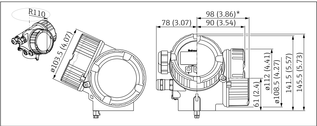
30 Housing GT20 (Alu coated); Dimensions in mm (in) *for devices with integrated overvoltage protection.
