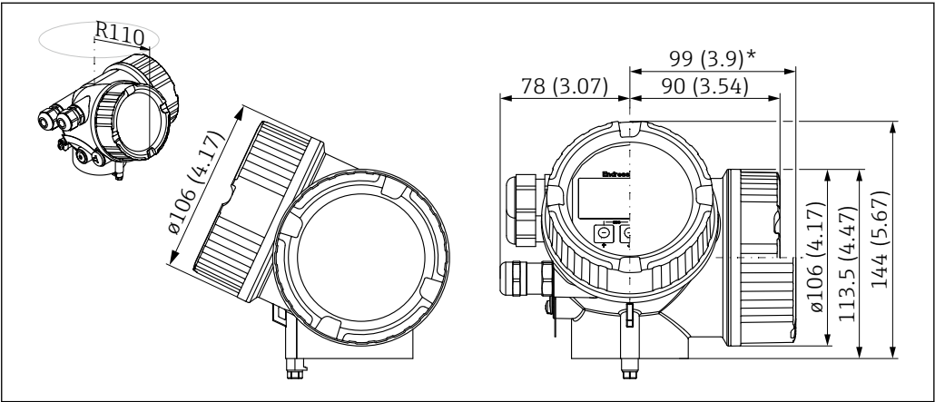
29 Housing GT19 (Plastics PBT); Dimensions in mm (in) *for devices with integrated overvoltage protection.
