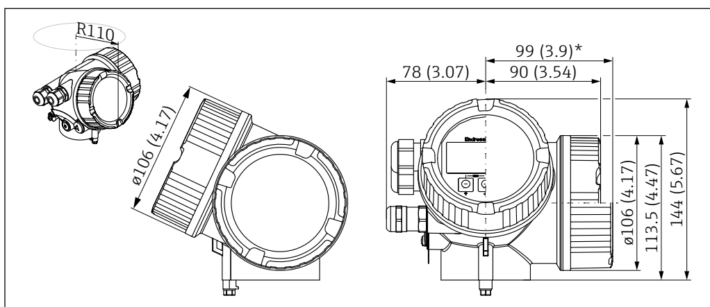
27 Housing GT19 (Plastics PBT); Dimensions in mm (in)
