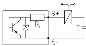
14 Connection of a relay
