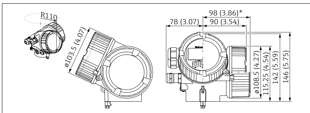
26 Housing GT18 (316L); Dimensions in mm (in)
