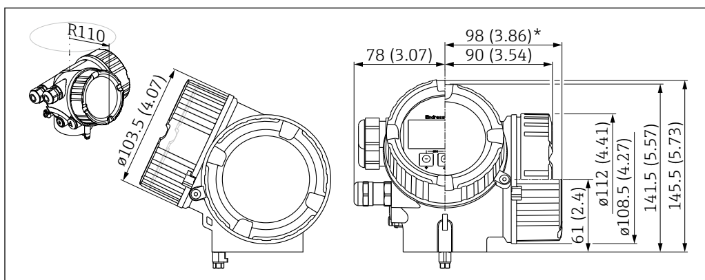
28 Housing GT20 (Alu coated); Dimensions in mm (in)
