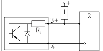
15 Connection of a digital input
