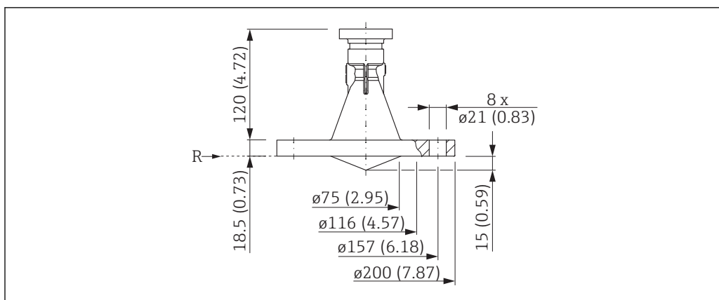
31 FMR56 with slip-on flange 3"/DN80; dimensions: mm (in)
