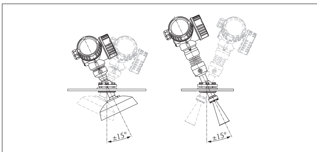
22 Micropilot FMR57 with alignment device
